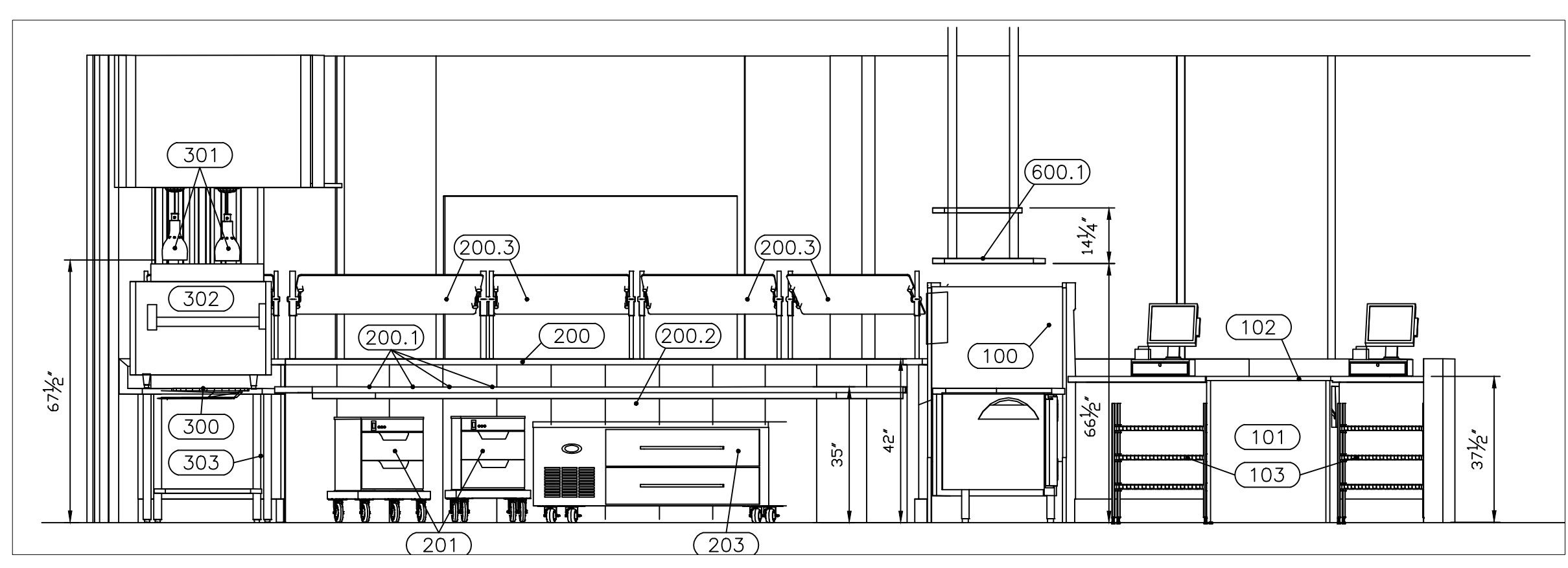
1 KITCHEN EQUIPMENT TAGGED PLAN K-401 SCALE: 3/8" = 1'-0"
