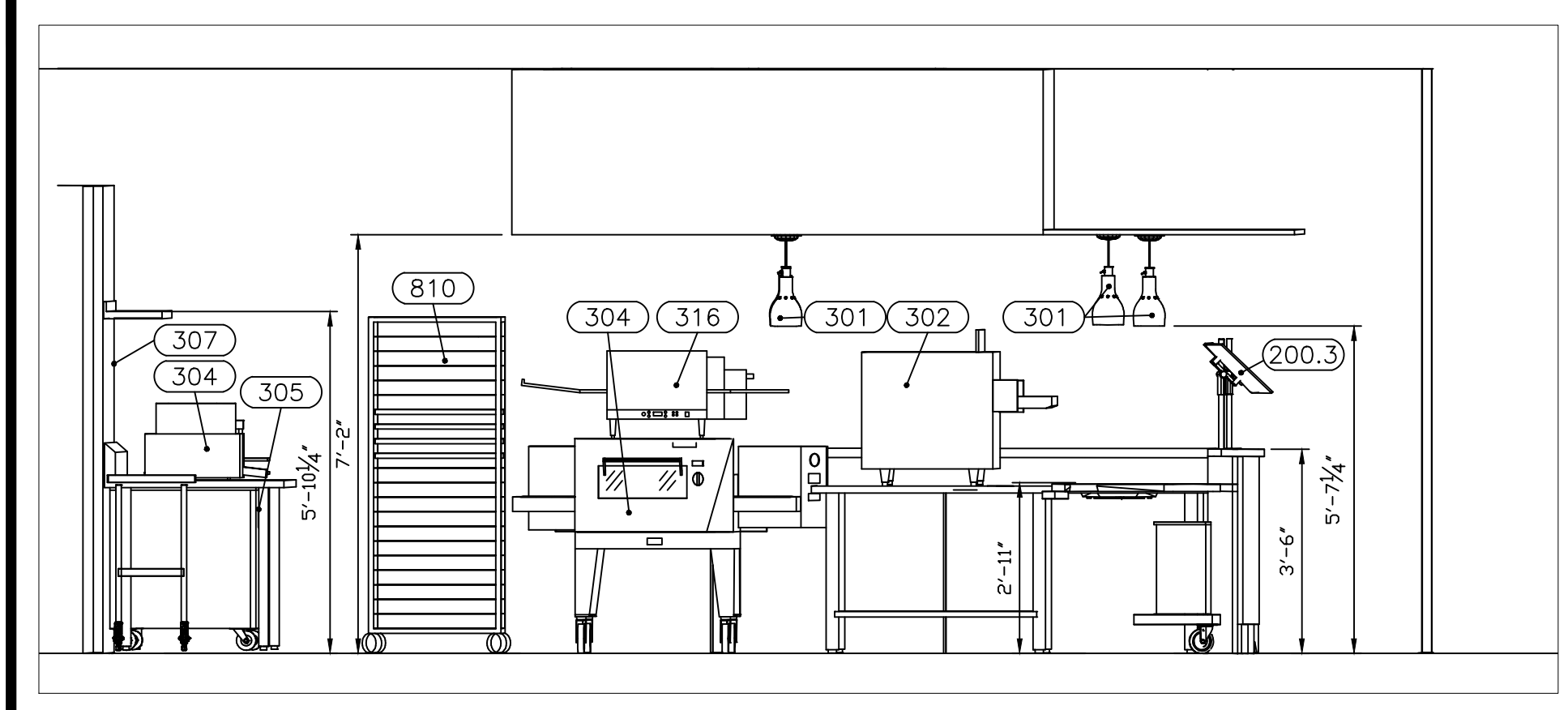
3 COOK LINE ELEVATION K-401 SCALE: 3/8" = 1'-0"
