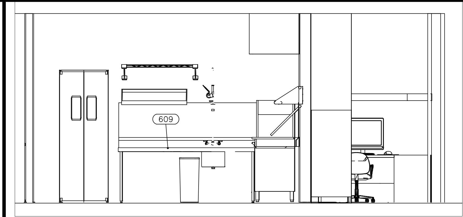
11 SOILED DISH ELEVATION K-401 SCALE: 3/8" = 1'-0"
