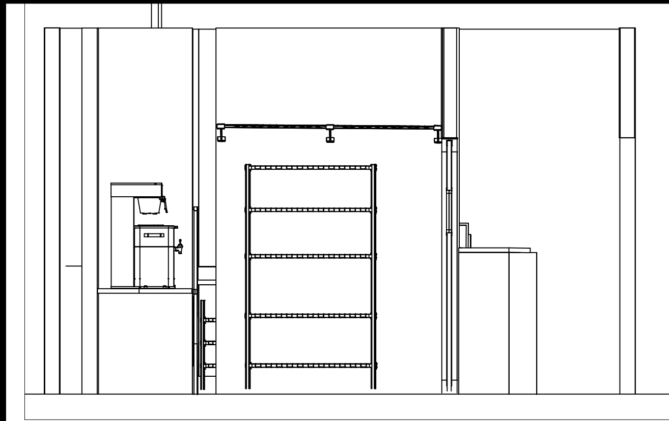
10 DRY STORAGE ELEVATION K-401 SCALE: 3/8" = 1'-0"
