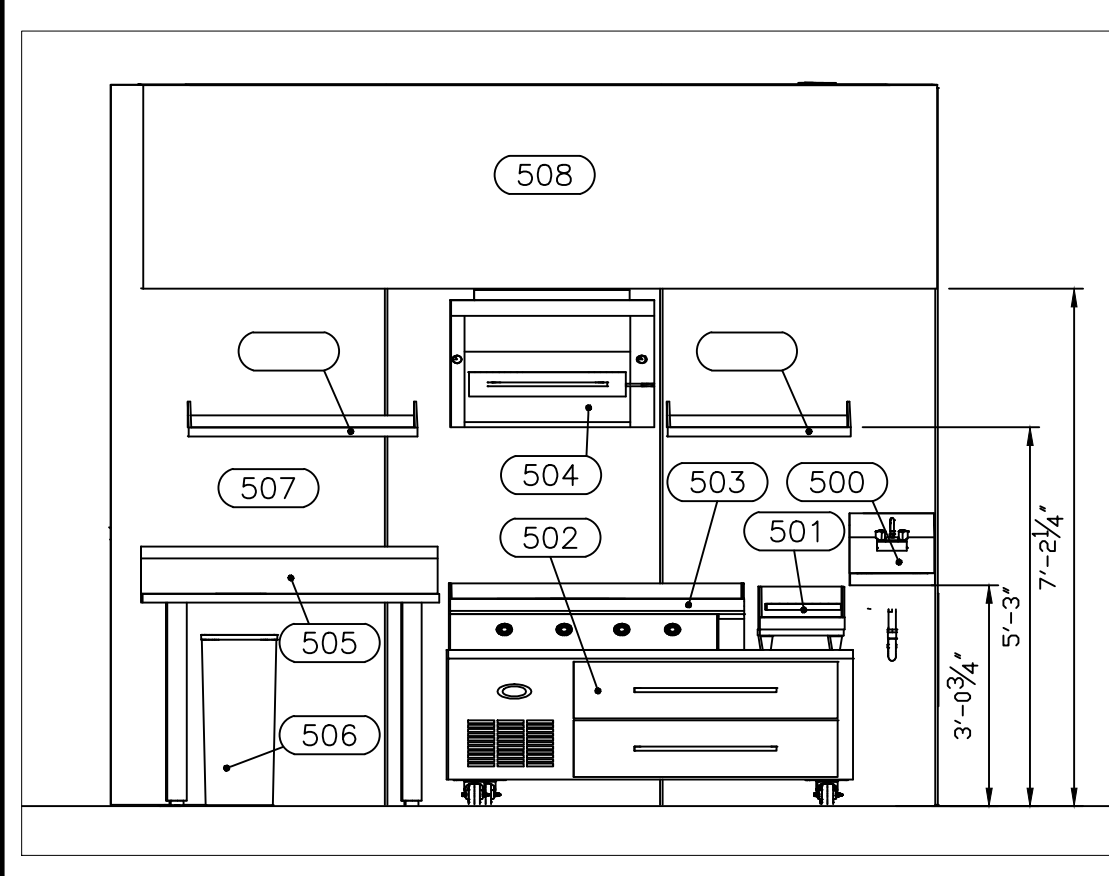
2 COOK LINE ELEVATION K-401 SCALE: 3/8" = 1'-0"
