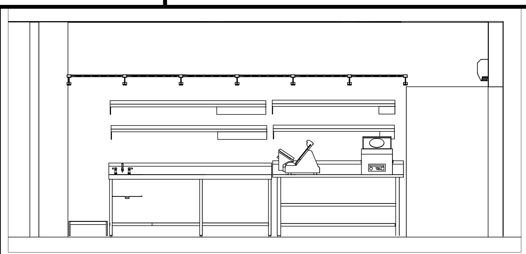
15 PREP STATION ELEVATION K-401 SCALE: 3/8" = 1'-0"
