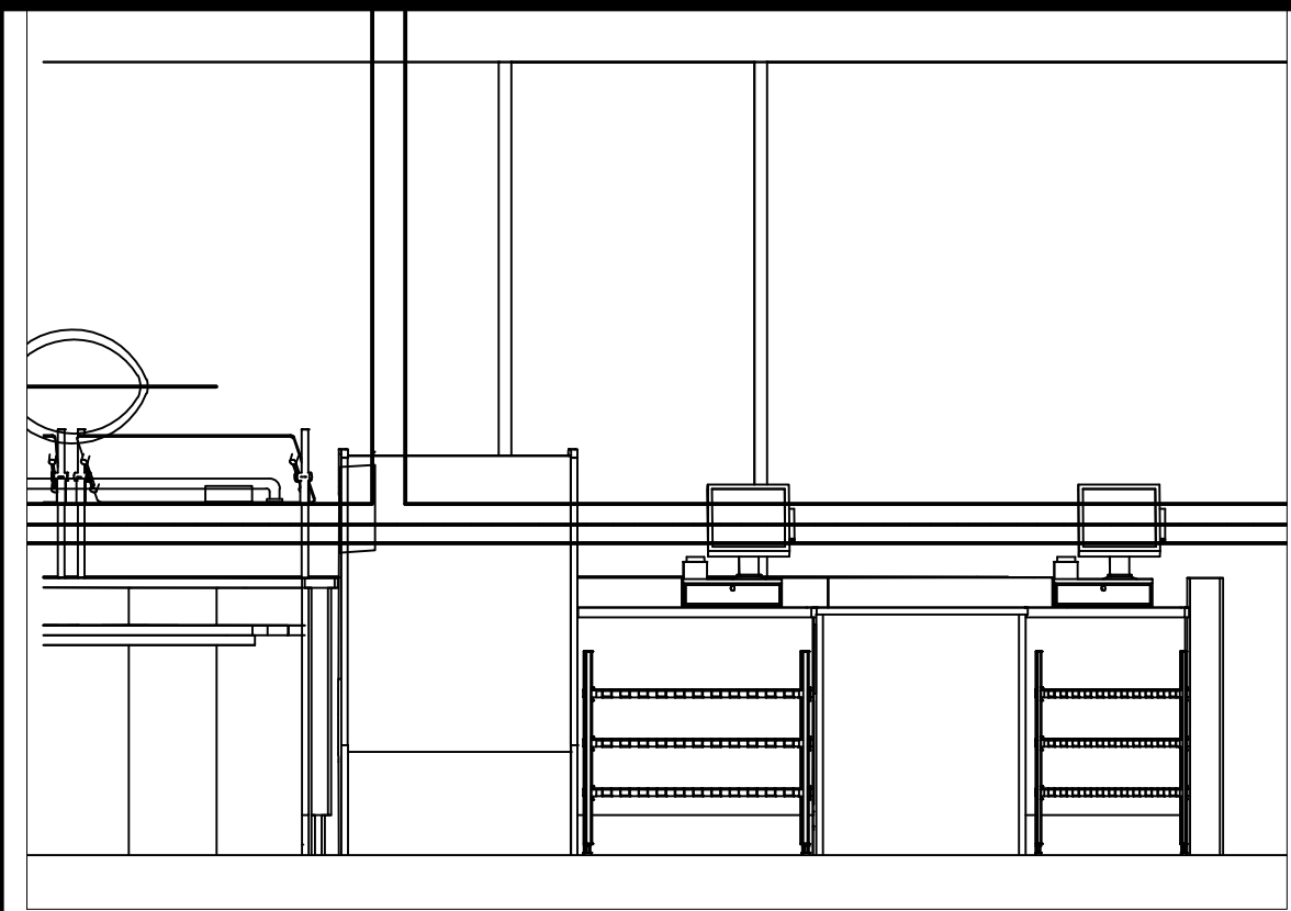
6 CASHIER ELEVATION K-401 SCALE: 3/8" = 1'-0"
